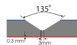
V shaped groove for 45° folding
